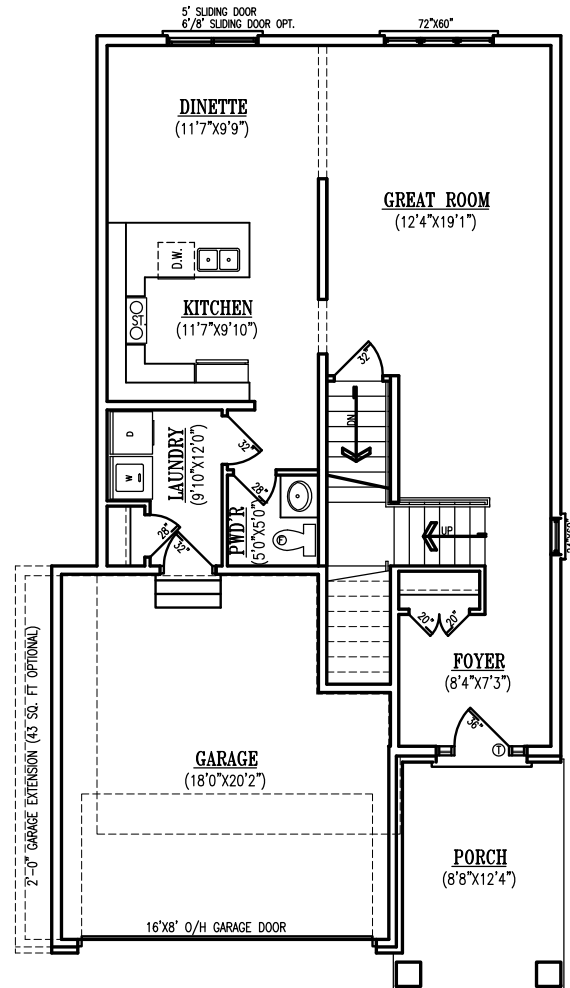
MAIN FLOOR PLAN 878 SQ. FT. (1960 SQ. FT. TOTAL) 81.56 SQ.M. (182.09 SQ.M. TOTAL)
