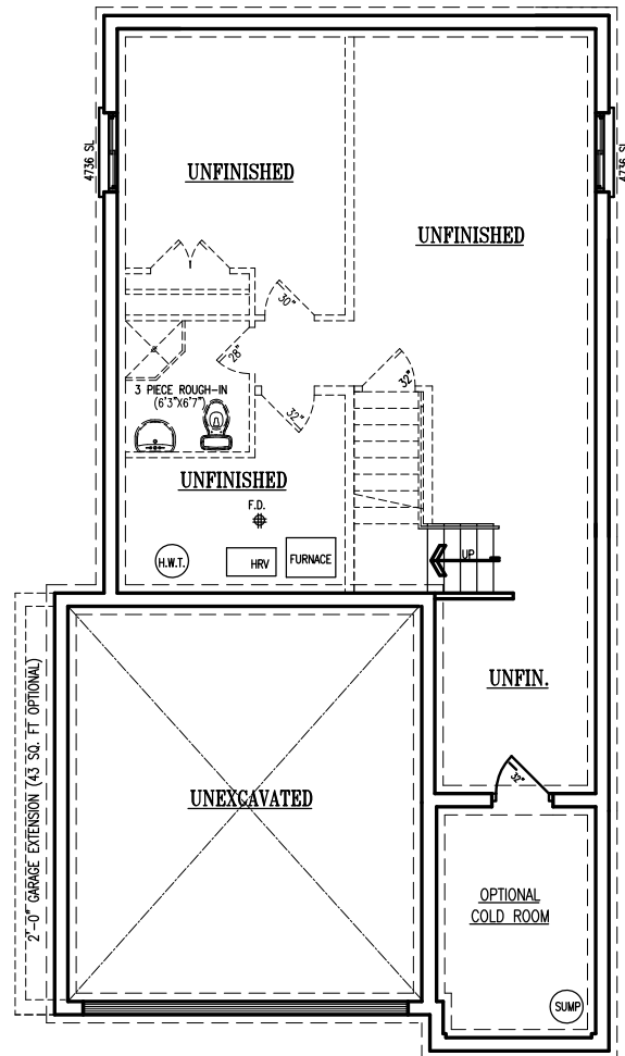
FOUNDATION PLAN
