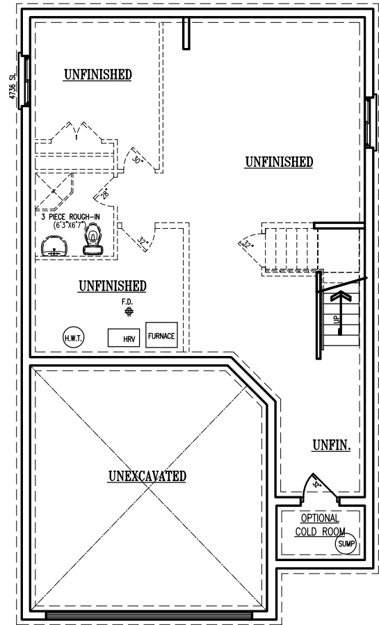
FOUNDATION PLAN
