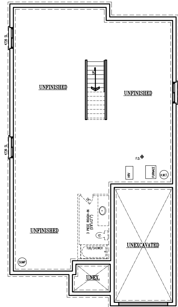
FOUNDATION PLAN
