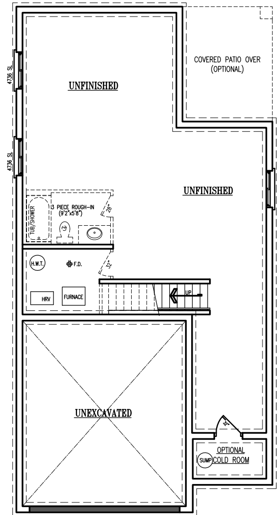
FOUNDATION PLAN
