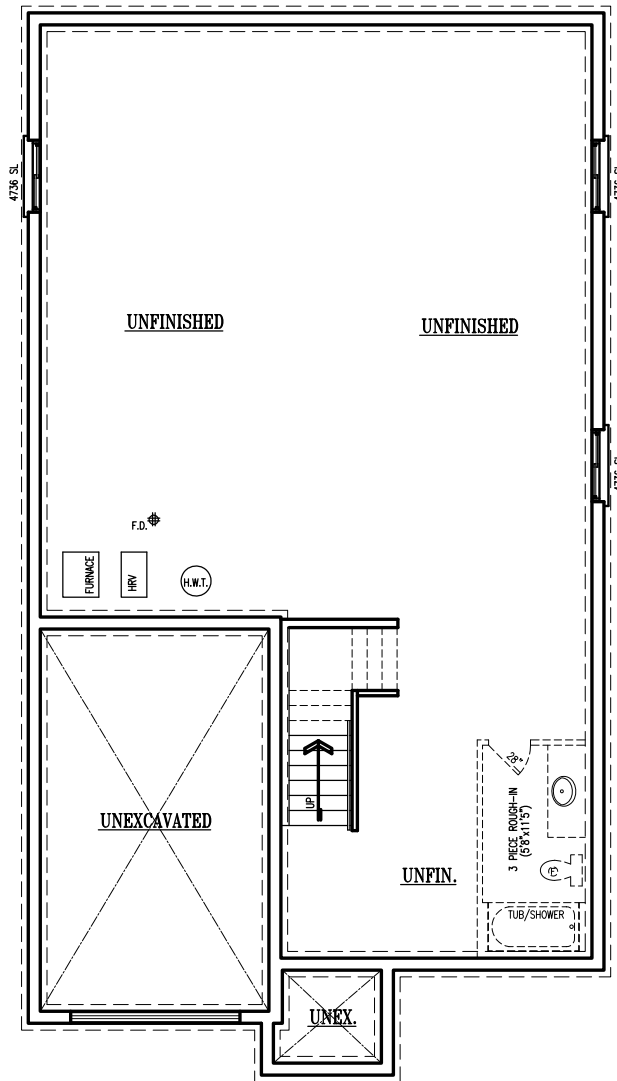
FOUNDATION PLAN
