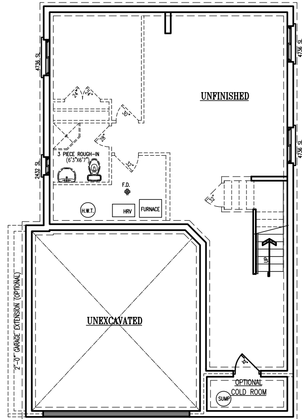
FOUNDATION PLAN
