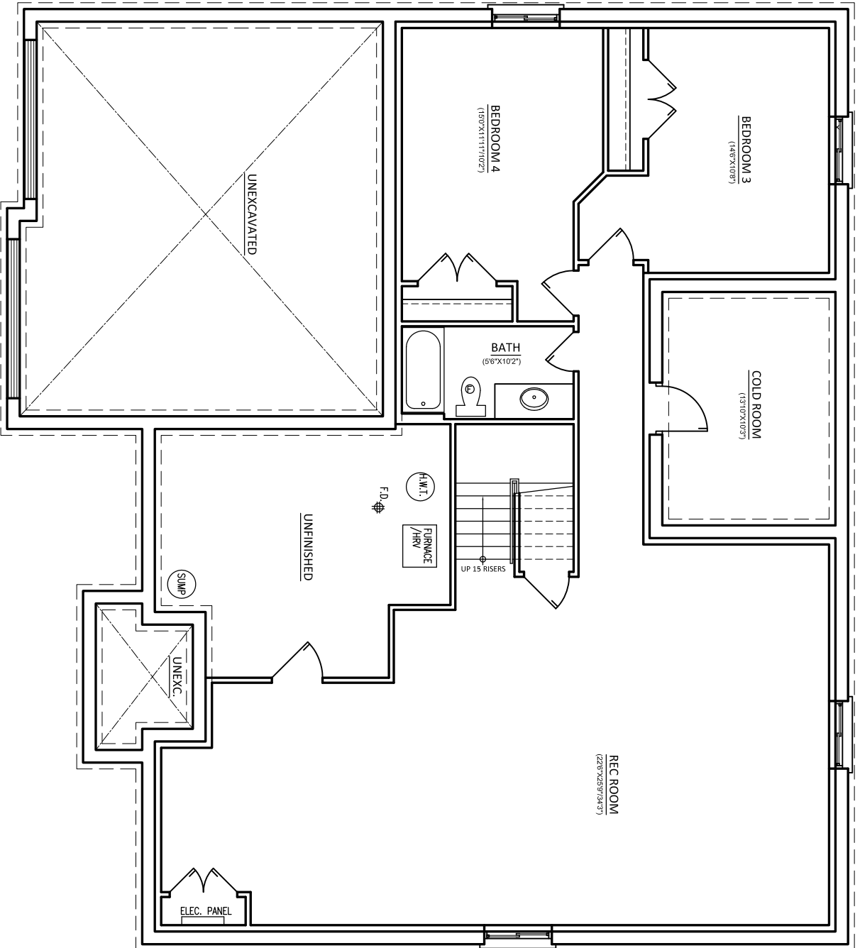
FOUNDATION PLAN 1342.45 SQ. FT. FINISHED (124.72 SQ.M.)
